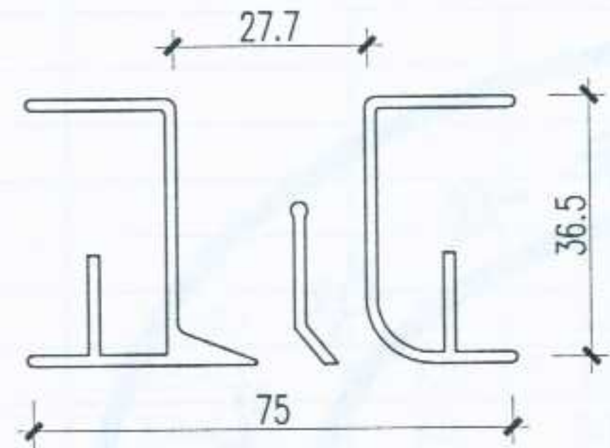
XS (单向气流型)
