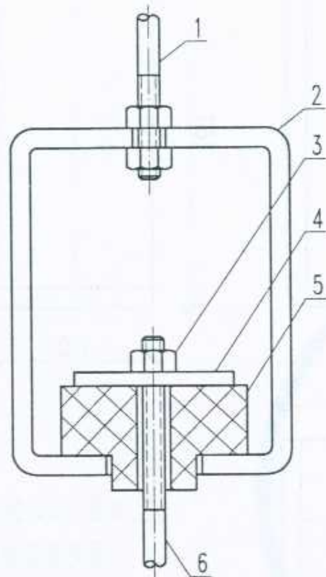
XTG型弹性吊架
