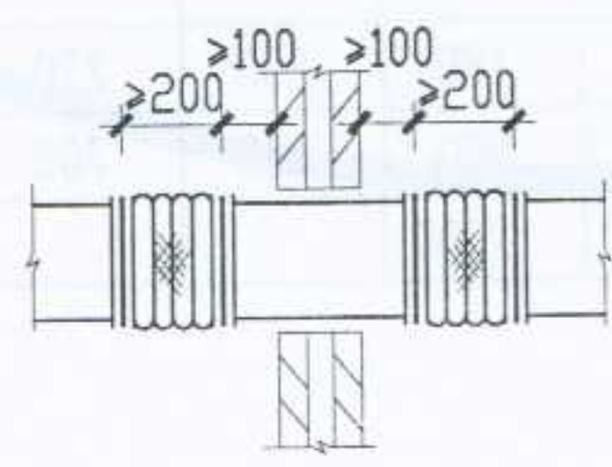
软管在伸缩缝处安装示意
